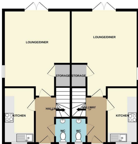
GROUND FLOOR 786 sq.ft. (73.1 sq.m.) approx.
